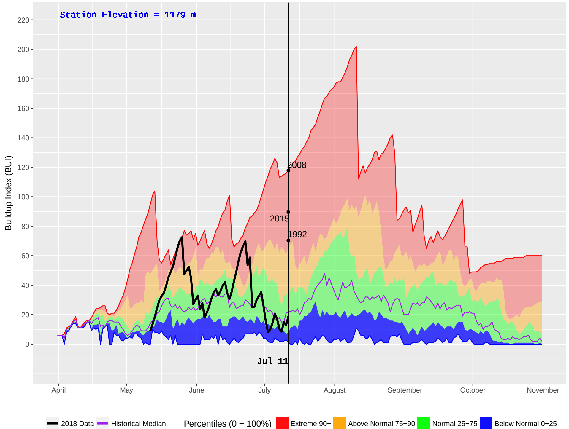
HOLMES (201) : Historical (1987–2016) and Current (2018) Noon Buildup Index (BUI)
