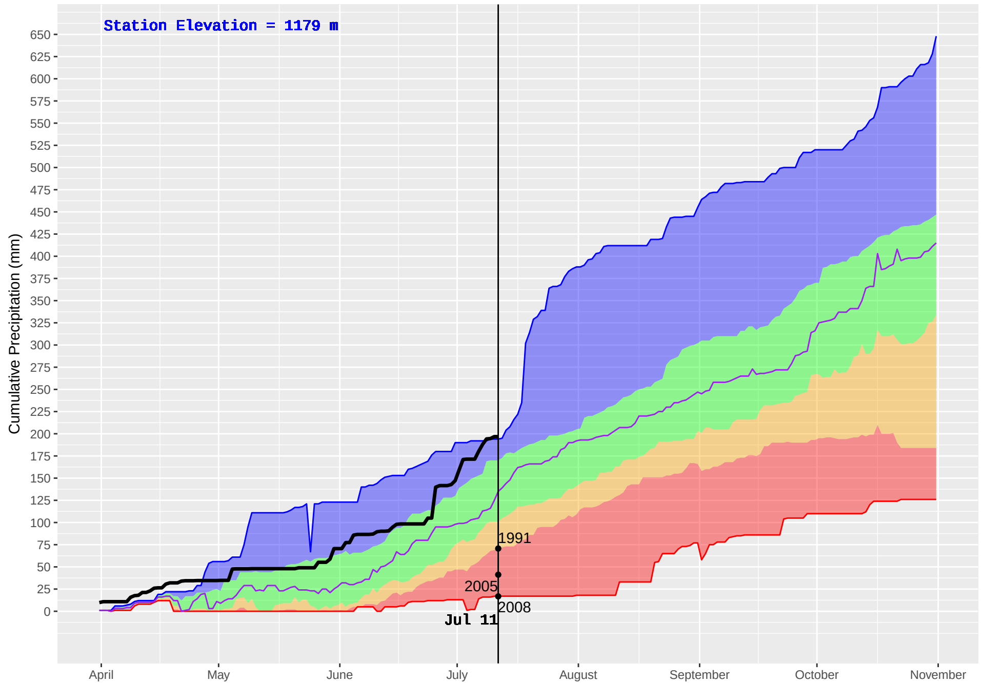
HOLMES (201) : Historical (1987–2016) and Current (2018) Noon Cumulative Precipitation
