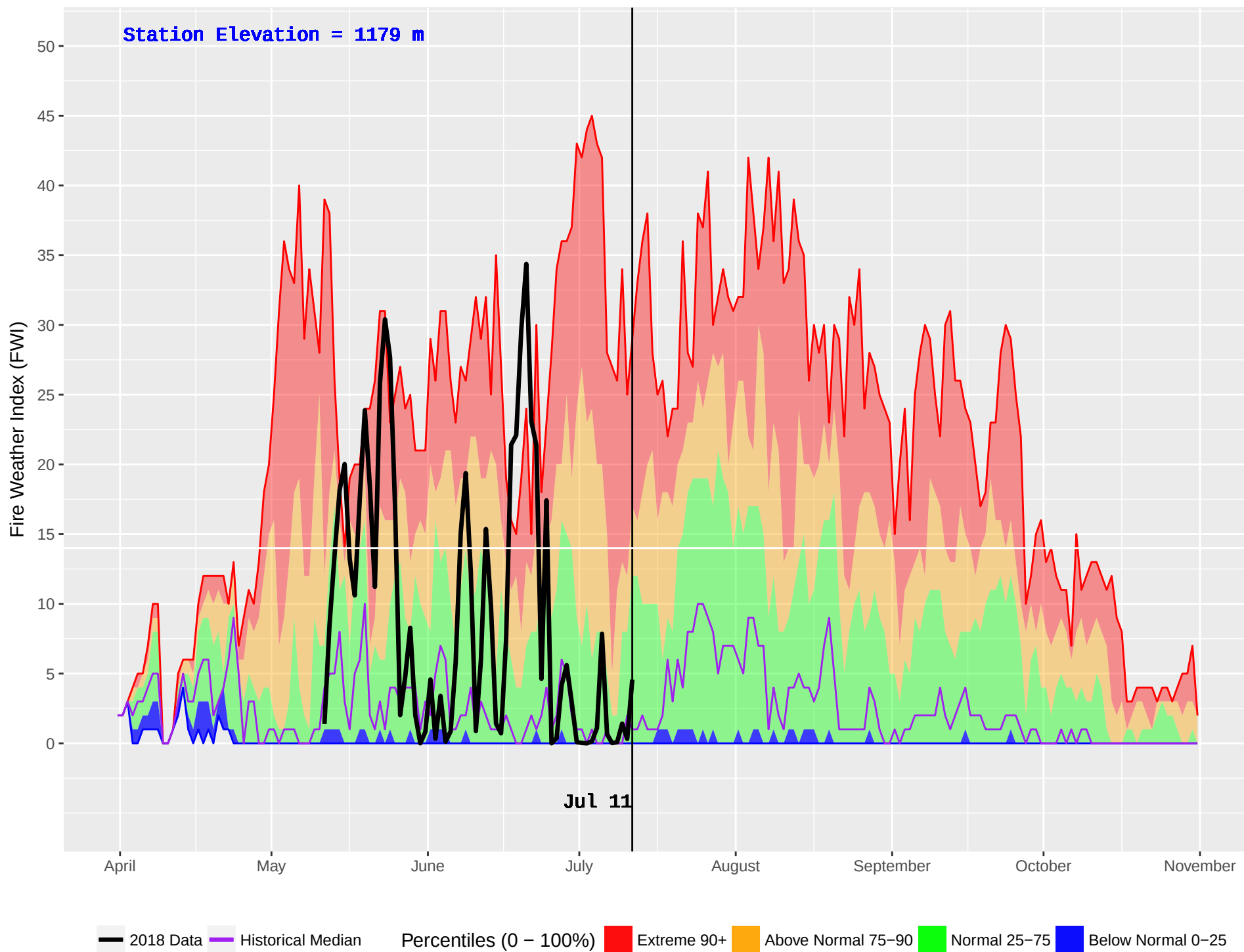
HOLMES (201) : Historical (1987–2016) and Current (2018) Noon Fire Weather Index (FWI)
