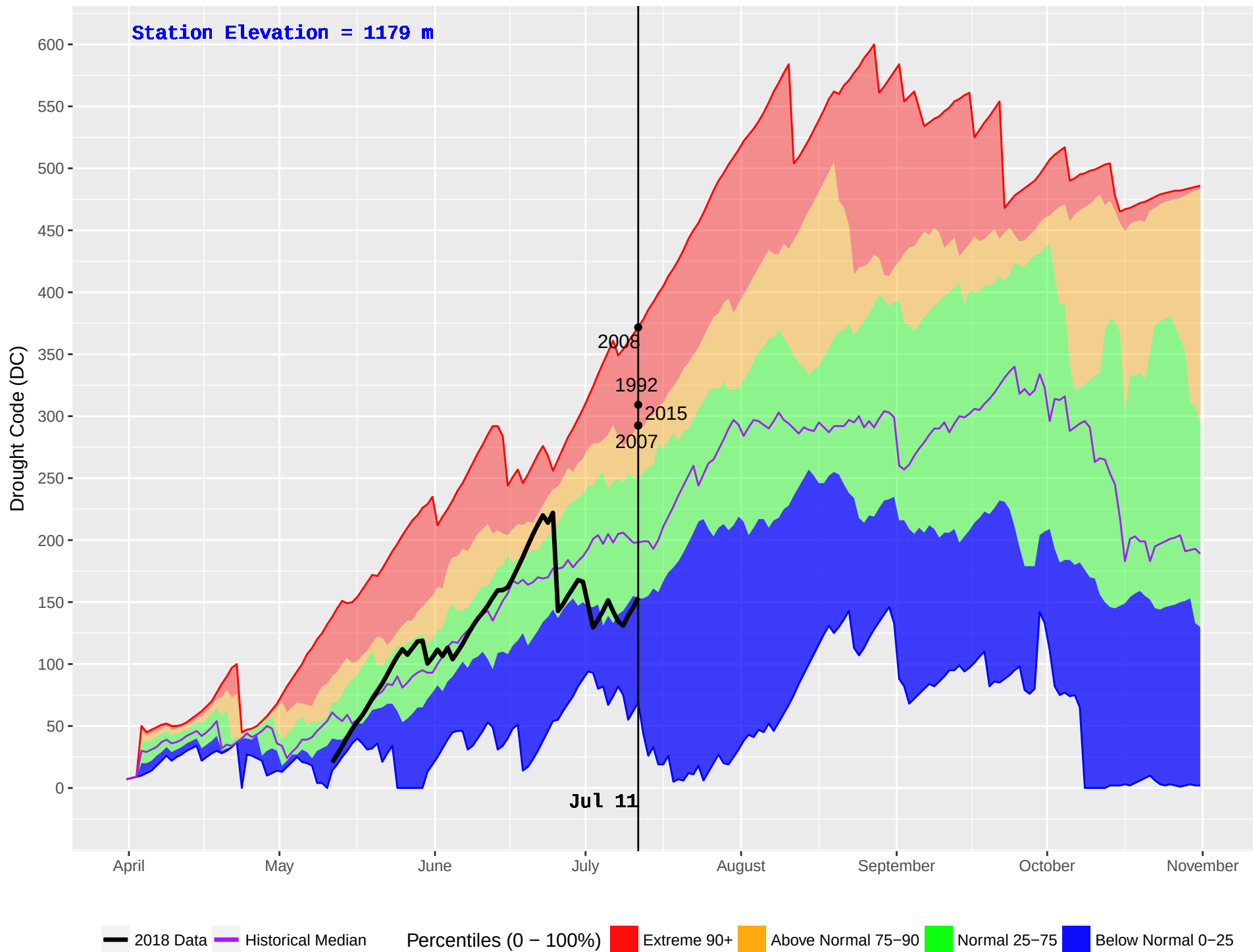
HOLMES (201) : Historical (1987–2016) and Current (2018) Noon Drought Code (DC)
