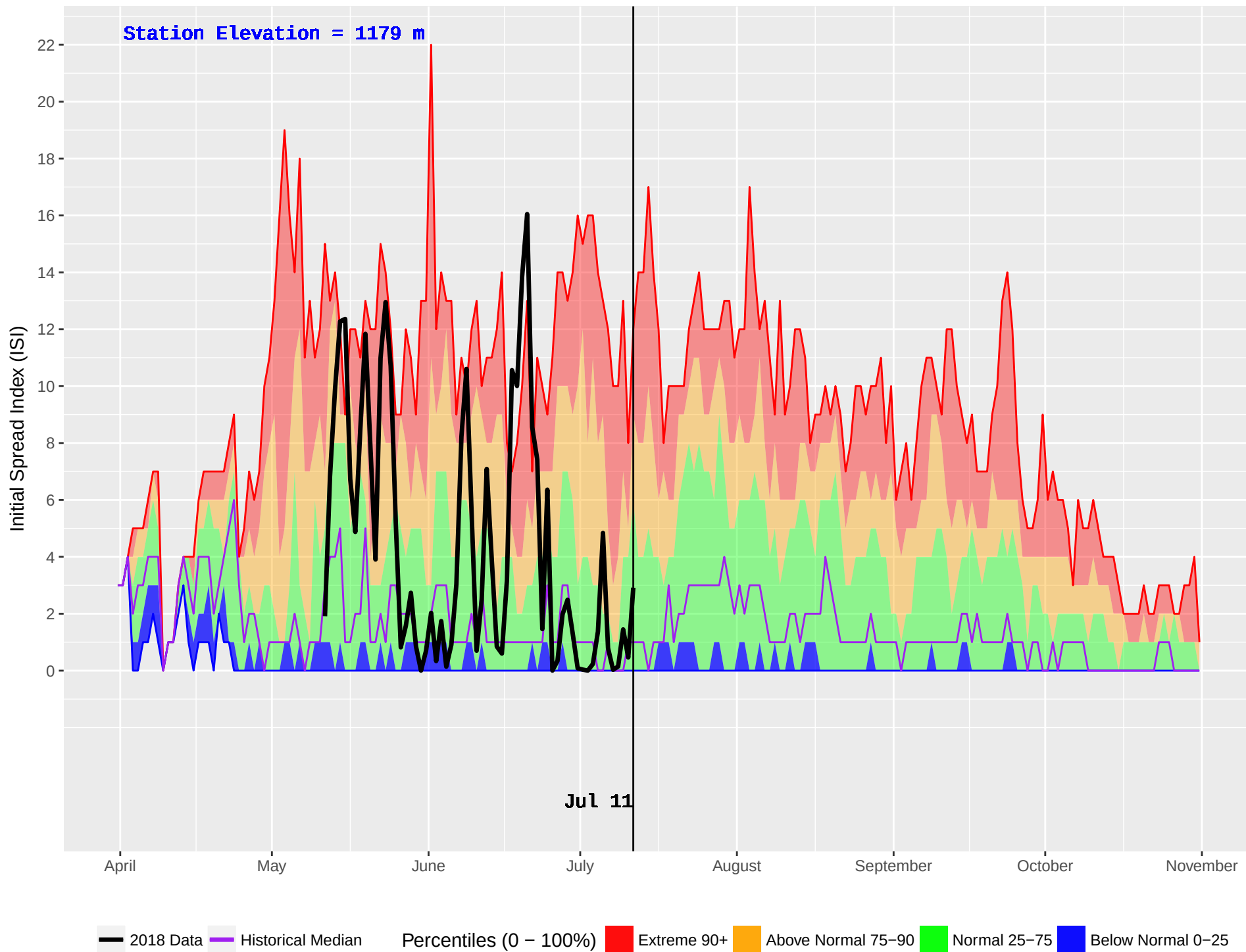
HOLMES (201) : Historical (1987–2016) and Current (2018) Noon Initial Spread Index (ISI)
