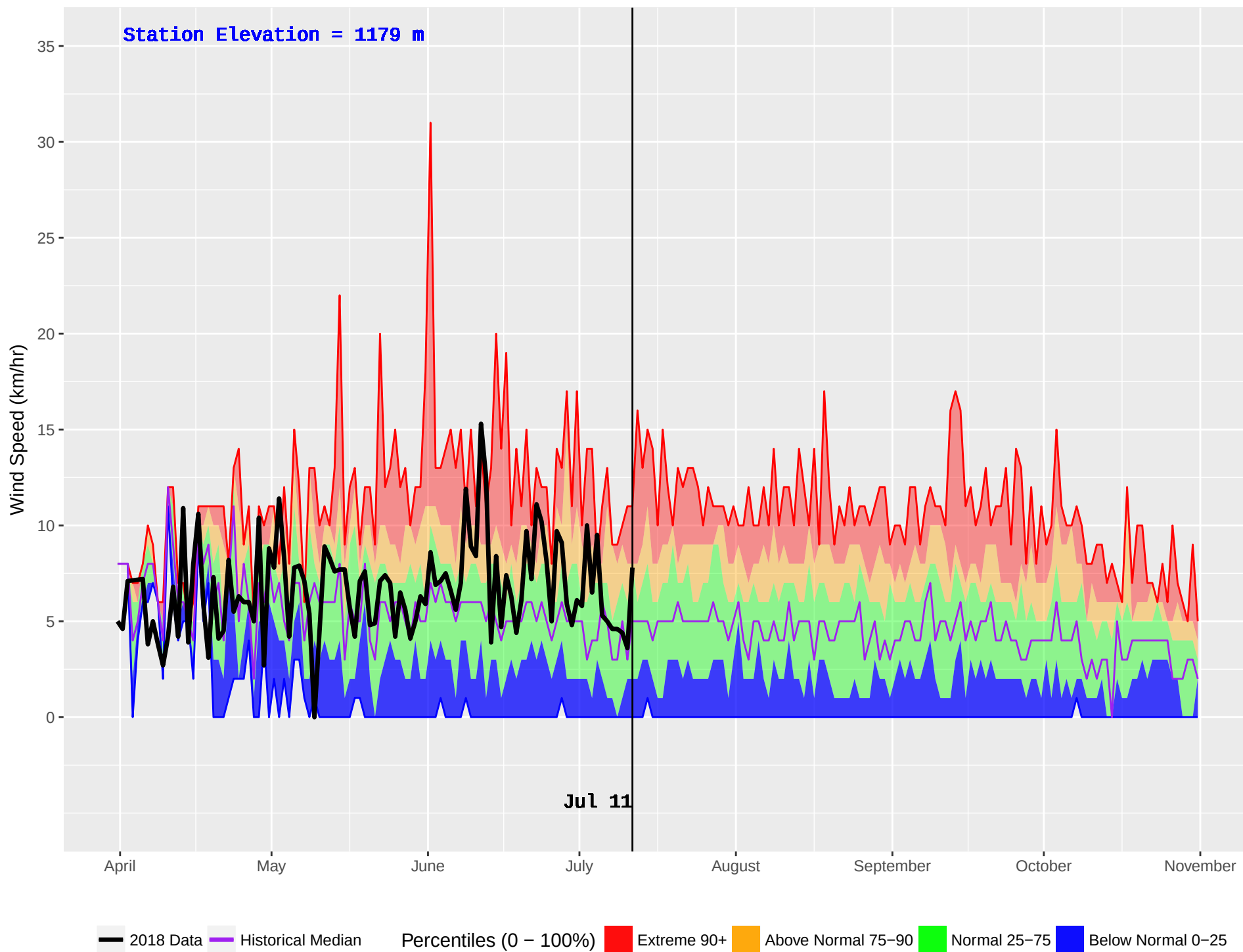
HOLMES (201) : Historical (1987–2016) and Current (2018) Noon Wind Speed
