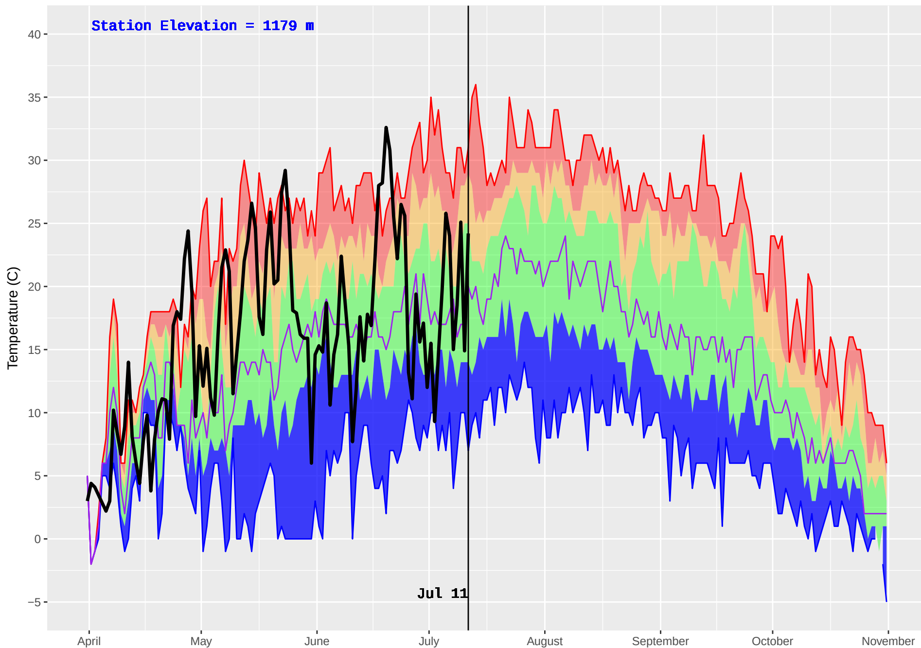
HOLMES (201) : Historical (1987–2016) and Current (2018) Noon Temperature
